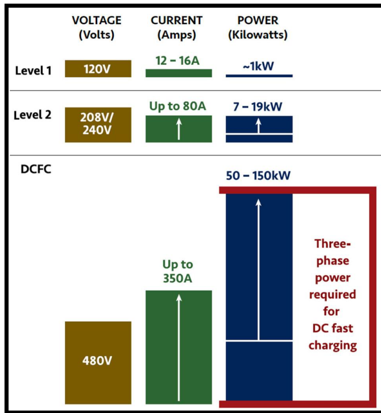
Figure 3: Electricity Needs for Different Charging Speeds (USDOT Volpe Center) i
