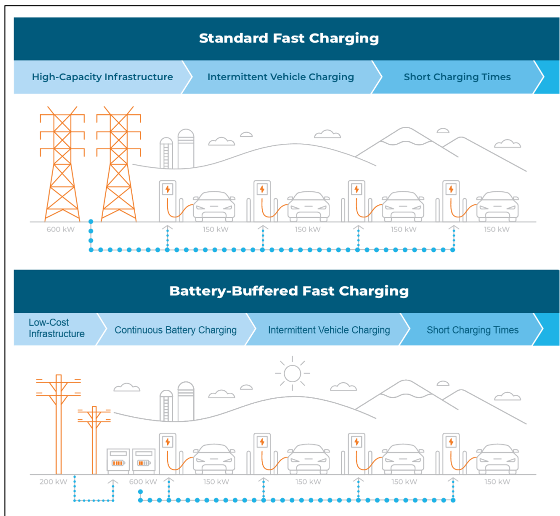
Figure 4: Standard vs Battery-Buffered Fast Charging (JOET) x
