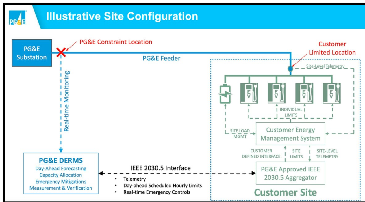
Figure 5: Illustrative Site Configuration (PG&E)
